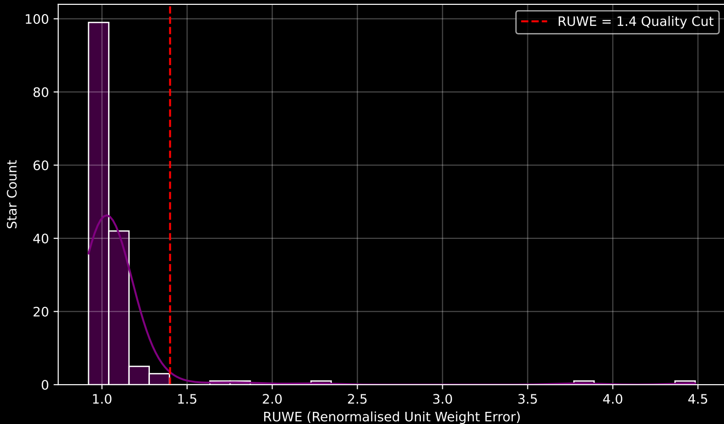
GAPOGEE DR17 Field [114-25_btx] RUWE Distribution (n= 154)
