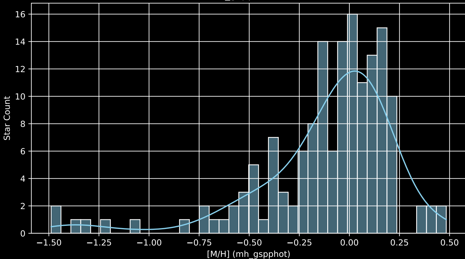
APOGEE DR17 Field: [114-25_btx [M/H] (mh_gspphot) (n= 153)
