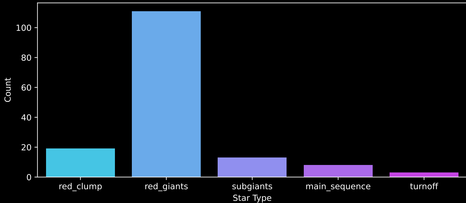
APOGEE DR17 Field: [114-25_btx] Count plot of Star Type
