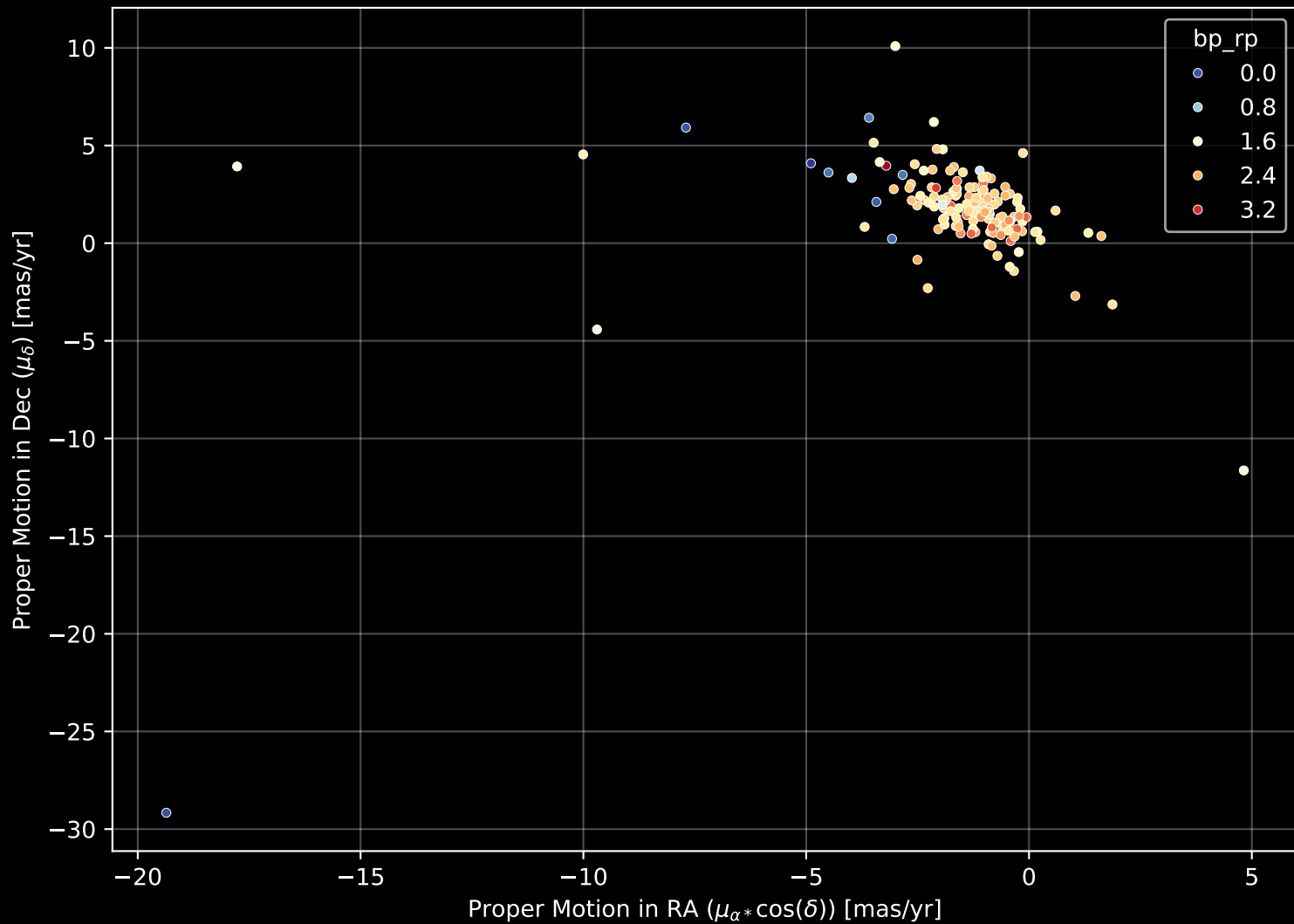
APOGEE DR17 Field: [114-25_btx] Proper Motion Diagram (n= 154)
