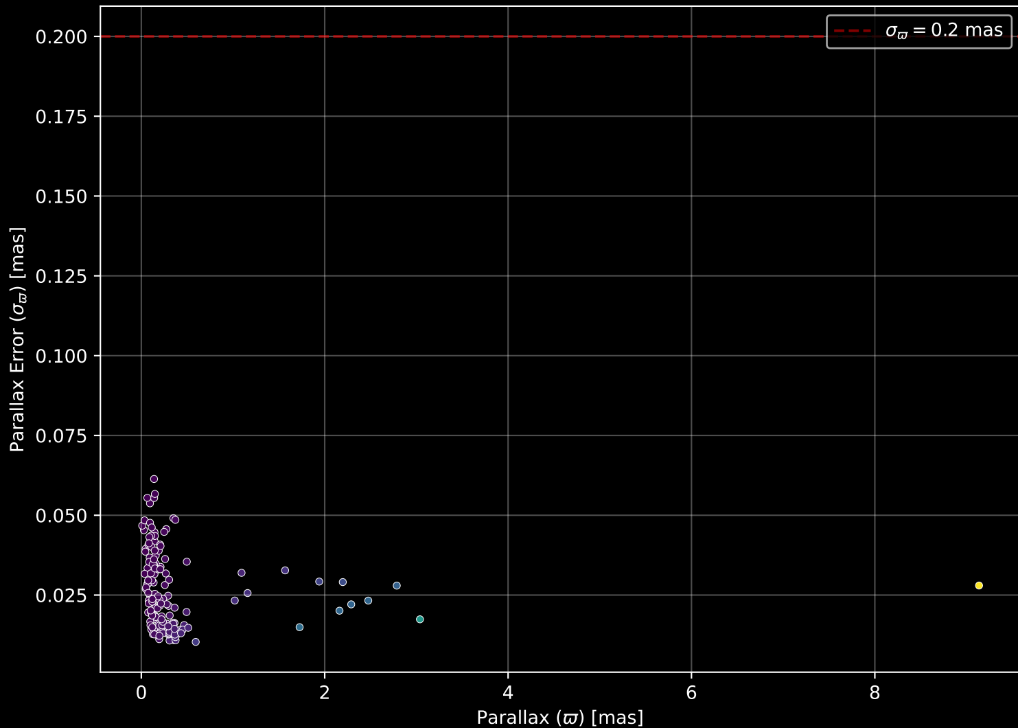
APOGEE DR17 Field: [114-25_btx] Parallax Quality (n= 154)
