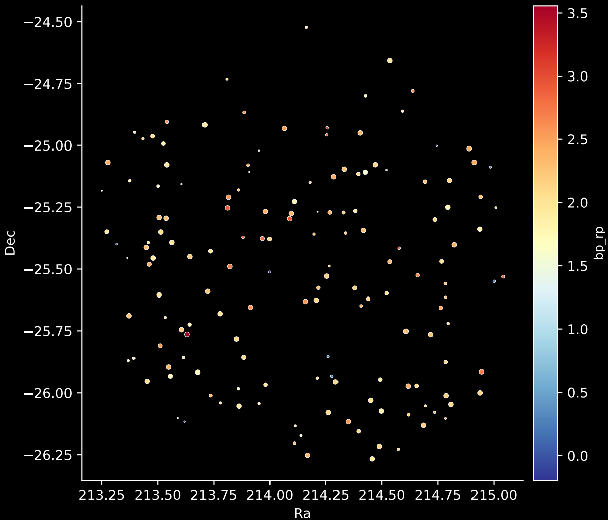
APOGEE DR17 Field: [114-25_btx] Stars: 154
